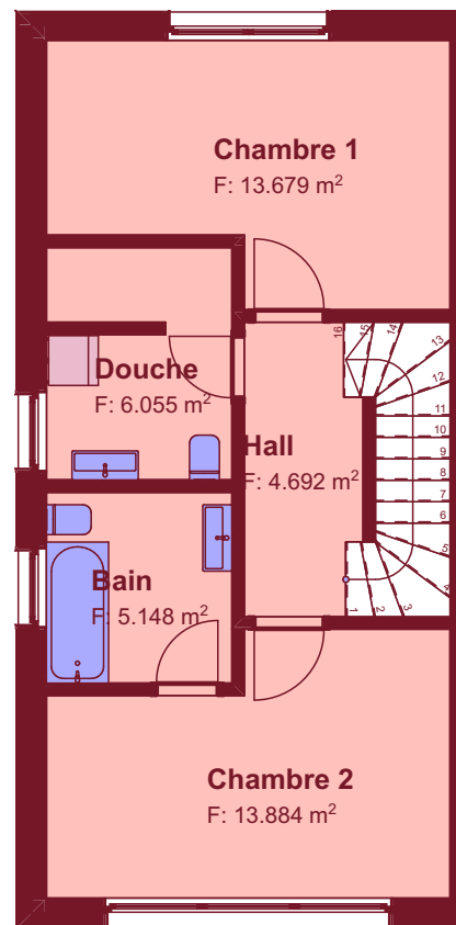
1. Story 1:100
