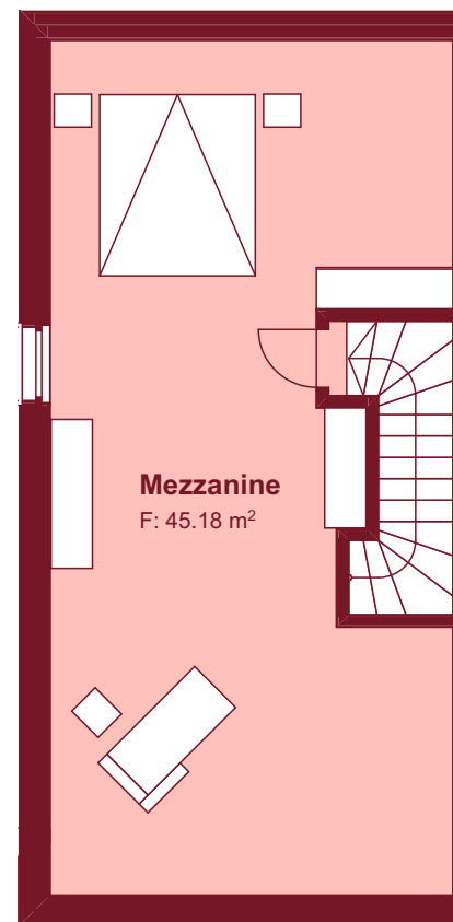
2. Story 1:100
